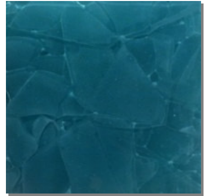
Emerald
